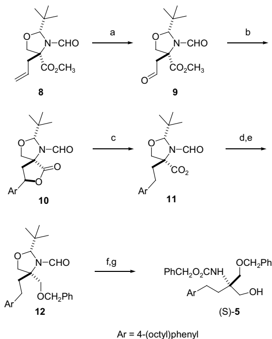
Scheme 2. (a) cat. OsO 4 , NaIO 4 , 3:1 v/v dioxane/H 2 O, rt (85%); (b) 4-(octyl)phenylmagnesium bromide, THF, −78 °C to rt (67%, ds = 1:1); (c) H 2 , 10% Pd/C, MeOH, rt (90%); (d) CH 3 CH 2 OCOCl, TEA, THF, 0 °C, then NaBH 4 , THF/H 2 O, 0 °C to rt (69%); (e) PhCH 2 Br, NaH, Bu 4 N + I − , DMF, 65 °C (93%); (f) 6.0N HCl, MeOH, reflux; (g) PhCH 2 OCOCl, KHCO 3 , EtOAc/H 2 O, rt (73%, 2 steps).
