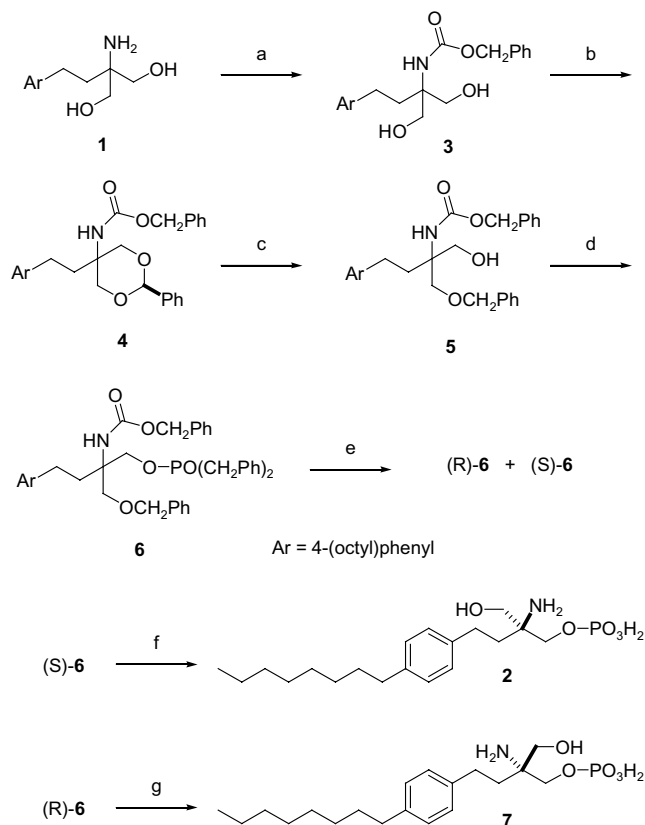
Scheme 1. (a) PhCH 2 OCOC 2 H 5 , KHCO 3 , EtOAc/H 2 O; (b) PhCHO, cat. p -TSA, toluene, 100 °C (57%, 2 steps); (c) BH 3 ·NHMe 2 , BF 3 ·OEt 2 , CH 2 Cl 2 , –78 °C → –5 °C (92%); (d) i Pr 2 N–P(OCH 2 Ph) 2 , 1 H -tetrazole, CH 2 Cl 2 , 0 °C, then MCPBA –78 °C → rt (99%); (e) enantiomer resolution (chiral HPLC); (f) TMS-I, CHCl 3 (63%); (g) Na, NH 3 , THF, –33 °C (81%).
